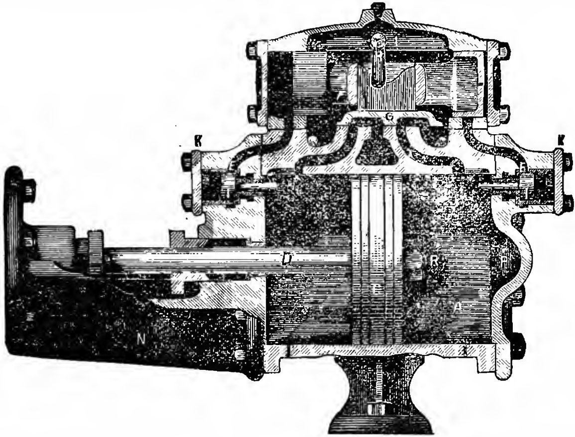
THE CAMERON STEAM PUMP. SECTIONAL VIEW OF STEAM CYLINDER.
